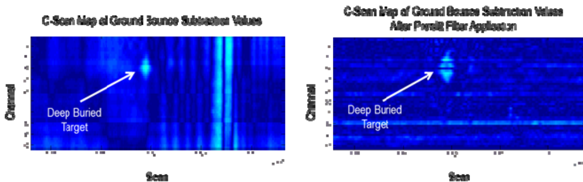
Figure 10. C-scan maps.
